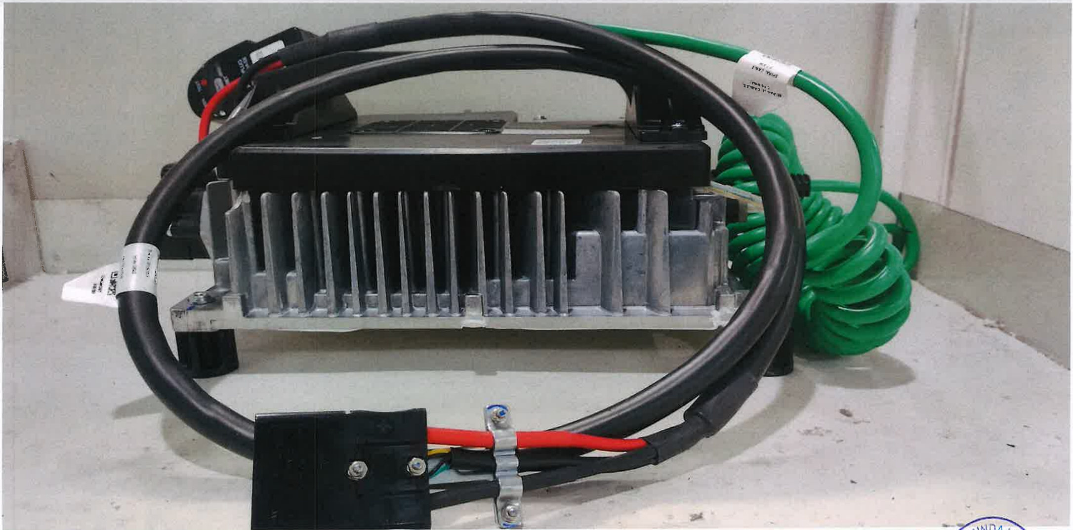
Portable Charger (Off Board Charger) 2200w – Photo Graph – Rear View
