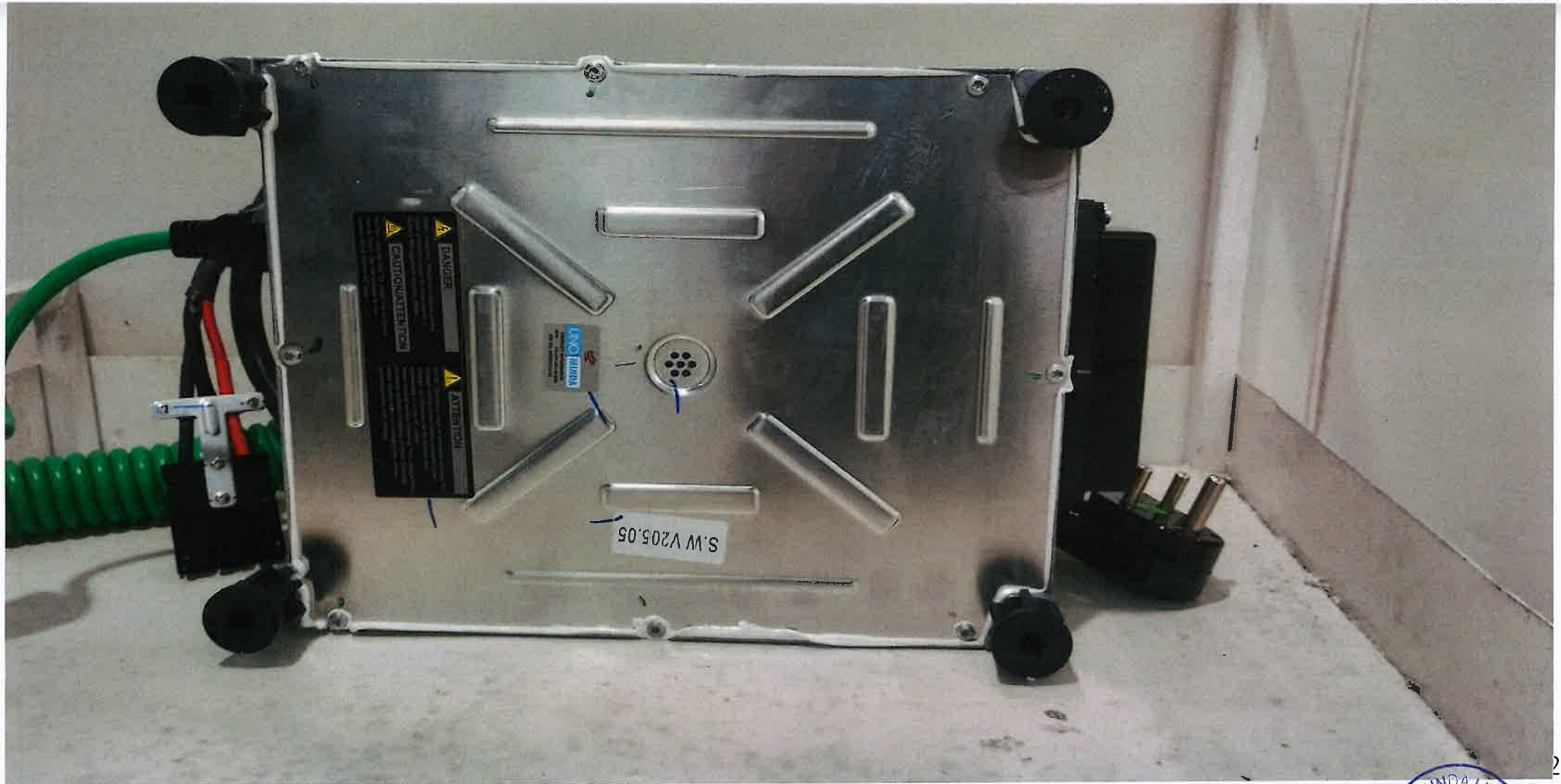
Portable Charger (Off Board Charger) 2200w – Photo Graph – Bottom View
